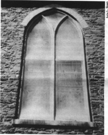
Figure 2: A typical example of polycarbonate protective glazing that has been in place ten years. The plastic has yellowed and become opaque as a result of the natural weathering process.
